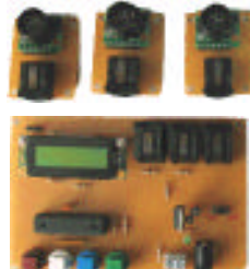
Ultrasoni Servo Tracker (BPE # UST-2088)
