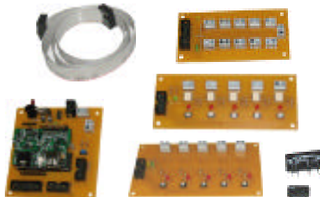
MP3 10-Ch Sound Board (BPE # MP3-2002)
